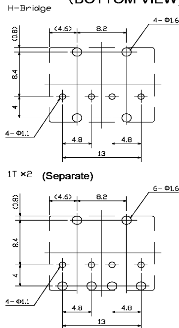
Fig.3. PCB pin layout (Reference figure) (BOTTOM VIEW)
